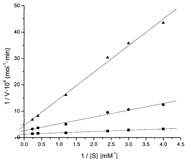
Fig. 3. Lineweaver-Burk plots for the inhibition of \alpha -D-glucosidase from jack bean (pH 5.25°) by (3R,4R)-1-(3-aminopropyl)pyrrolidine-3,4-diol ( 10j ). ■ = 0 \mu M (control), ● = 16 \mu M, ▲ = 32 \mu M.
